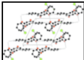
Fig. 2. The packing of the title compound, viewed down the a axis. Dashed lines indicate hydrogen bonds. H atoms not involved in hydrogen bonding have been omitted.
